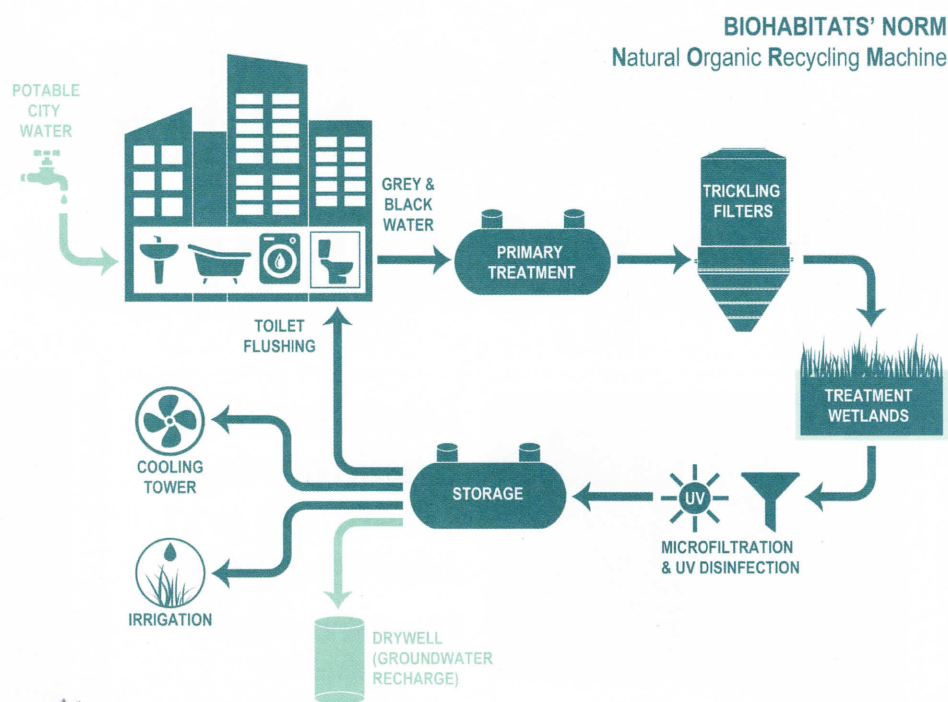
Hassalo on 8th system schematic. Courtesy of Biohabitats, Inc.
