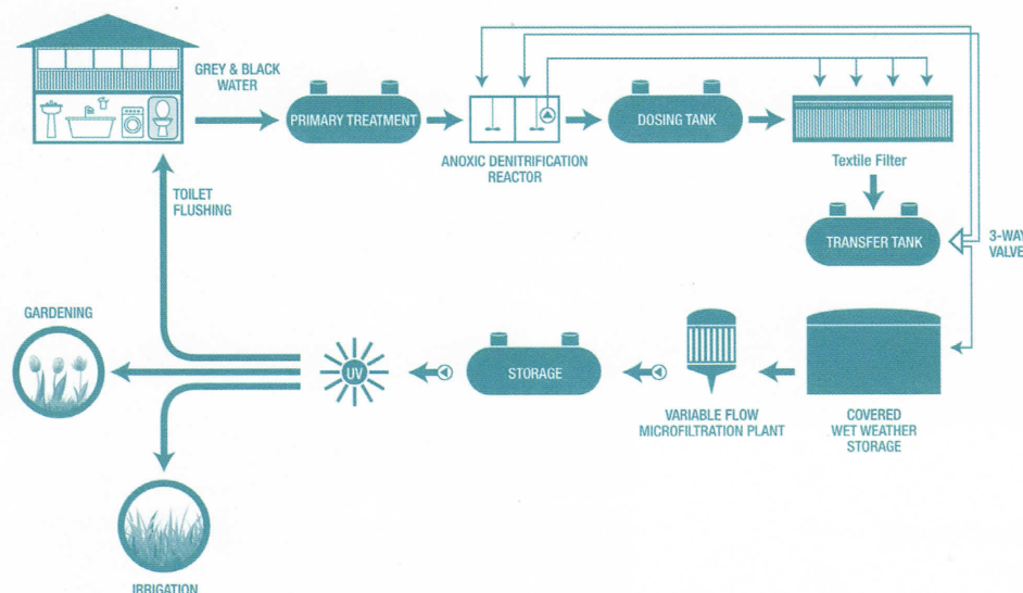
Left: Ecovillage system schematic. Image provided by Orenco Systems, Inc.
