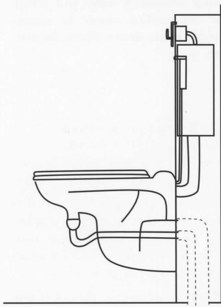
Figure 7. Side view of the wall-hung Dubbletten model with a toilet seal for the urine pipe.
