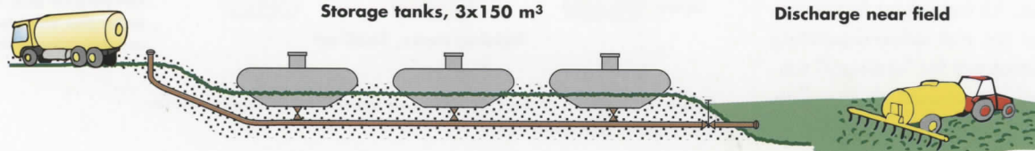
Figure 6. Diagram of the storage facility for human urine at Lake Bornsjön. Illustration: Kim Gutekunst
