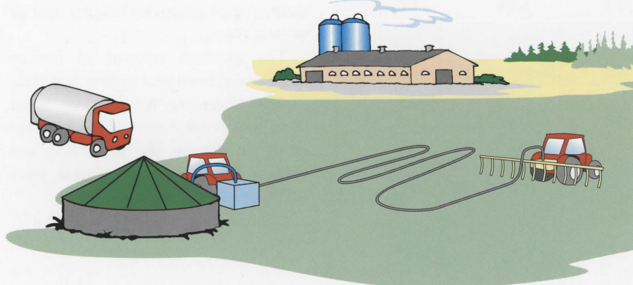
Figure 12. The fertilizer is pumped through a feeder hose system out to an applicator drawn by a tractor. This substantially reduces the damage to soil and crops since a heavy tank wagon is not used to spread the fertilizer in the field.
