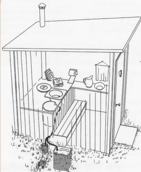
Urine-separating inset for dry closets.
