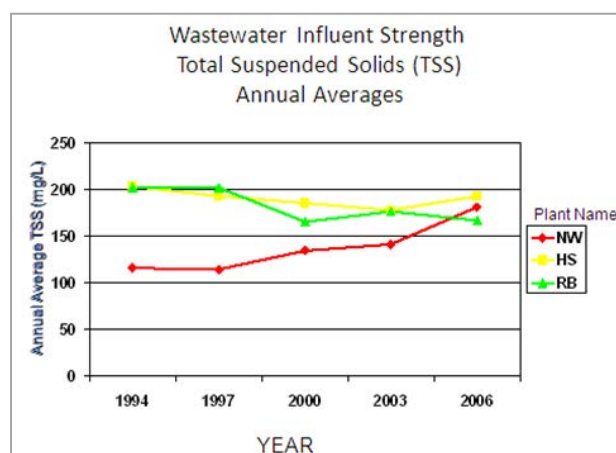
Figure 5-29 Wastewater influent strength, TSS
