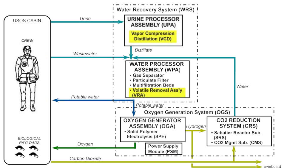
Figure 1 WRS and Oxygen Generator Assembly (OGS) process flow diagram
