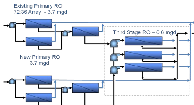
Figure 4 Three stage RO system (Photo credit: SPI 2011)
