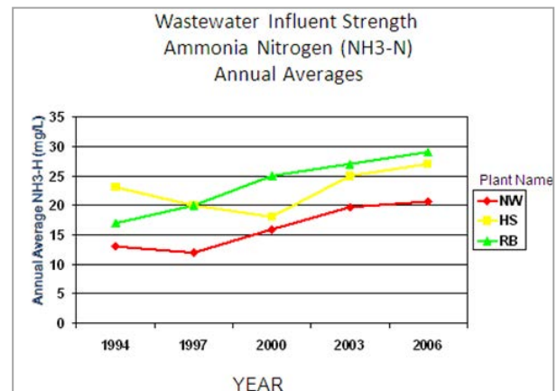
Figure 5-28 Wastewater influent strength, NH 3 -N
