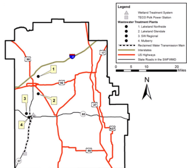
Figure 2 Project location
